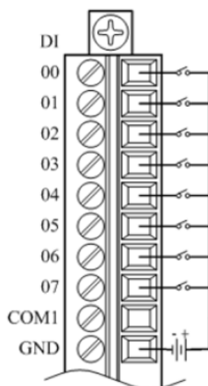
Dry Contact Wiring
