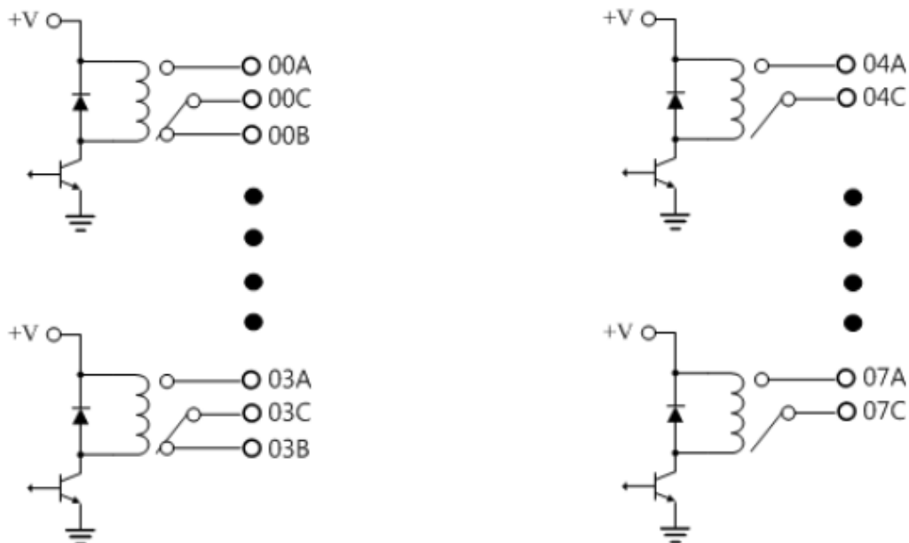
Block Diagram
